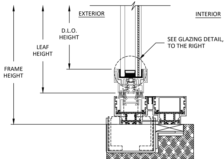
B 5 VERTICAL SECTION SILL
